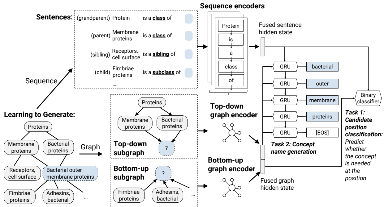
Figure 3: Architecture of GENTAXO. Suppose the concept “bacterial outer membrane proteins” is masked. Given the masked position in the taxonomy, the model learns to generate the name of the concept. It has two types of encoders to represent the relational contexts of the position. Sequence encoders learn a group of sentences that describe the relations with the masked concept. Graph encoders learn the masked concept’s embedding by aggregating information from its top-down and bottom-up subgraphs. The fused sentence- and graph-based hidden states are used to predict whether the masked position is valid (Task 1). They are fed into GRU decoders to generate the concept’s name (Task 2).
