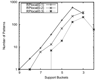
Figure 22: Number of Output Patterns w.r.t. Support Buckets, Accidents Data Set
