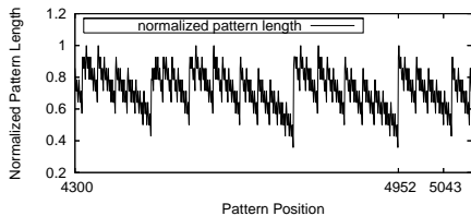
Figure 6: Patterns' Positions and Their Length
