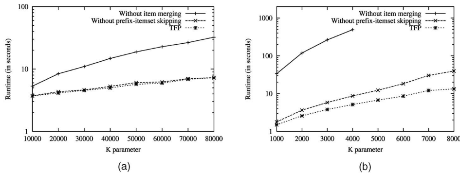
Fig. 8. Search space pruning method evaluation ( min\_l = 10 ). (a) Connect-4 data set. (b) Gazelle data set.
