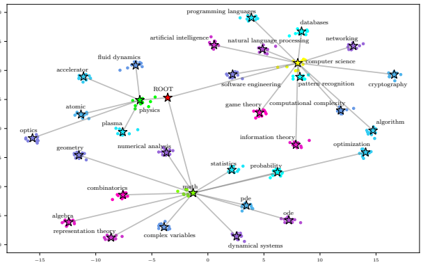
(b) arXiv joint embedding space.
