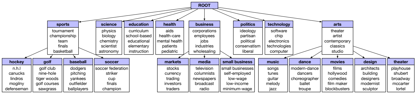
Figure 3: Hierarchical Topic Mining results on NYT.
